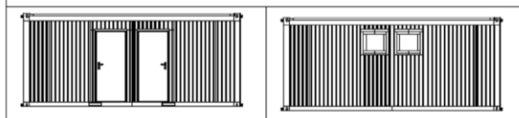
Changing Room, Toilet, Social and Refreshment Area Two Side Elevation Viewpoints - Scale 1:50
